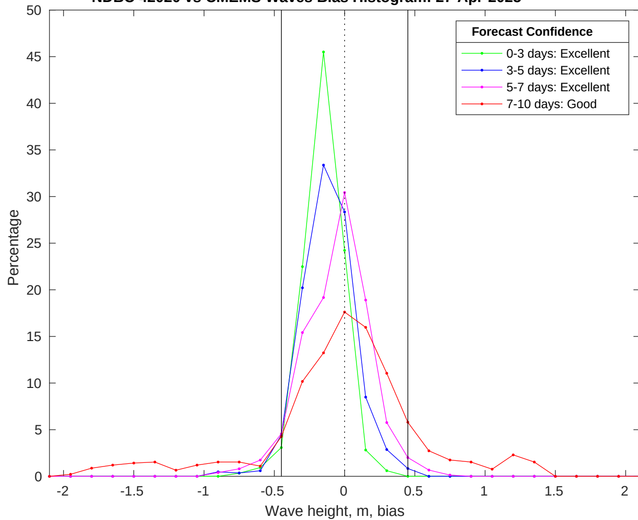
NDBC 42020 vs CMEMS Waves Bias Histogram: 27-Apr-2025
