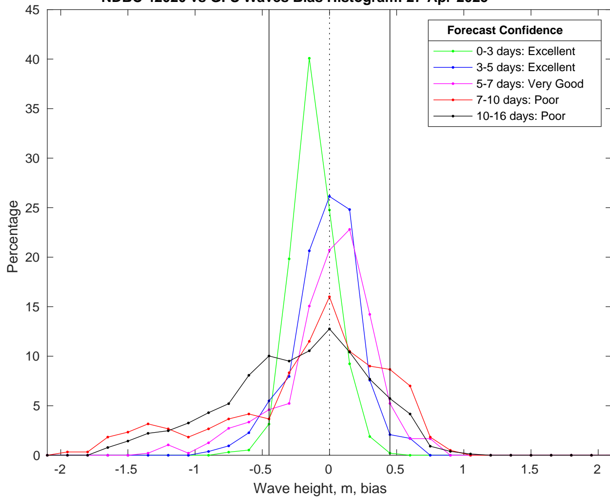
NDBC 42020 vs GFS Waves Bias Histogram: 27-Apr-2025
