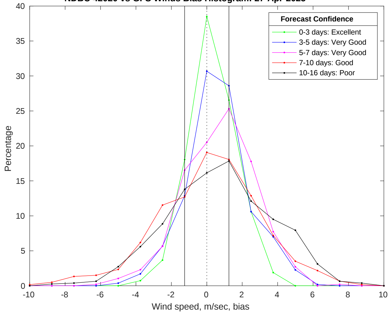
NDBC 42020 vs GFS Winds Bias Histogram: 27-Apr-2025
