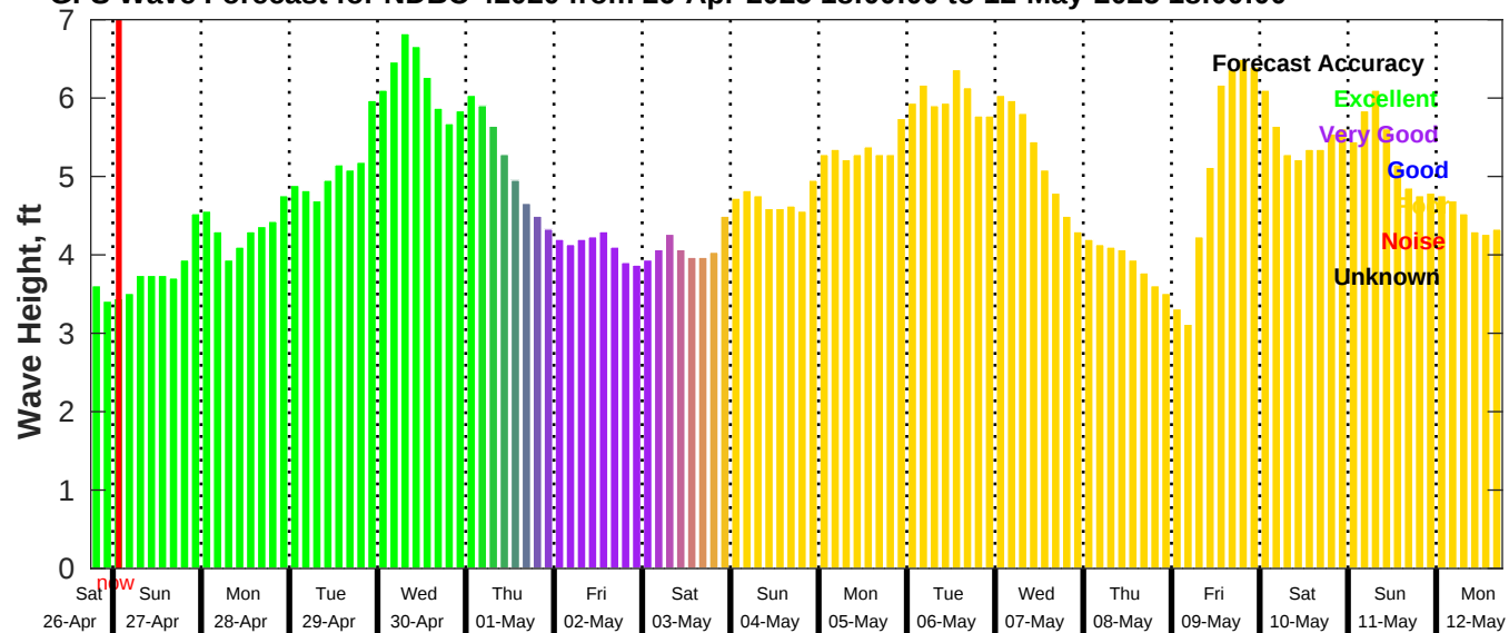
GFS Wave Forecast for NDBC 42020 from 26-Apr-2025 18:00:00 to 12-May-2025 18:00:00
