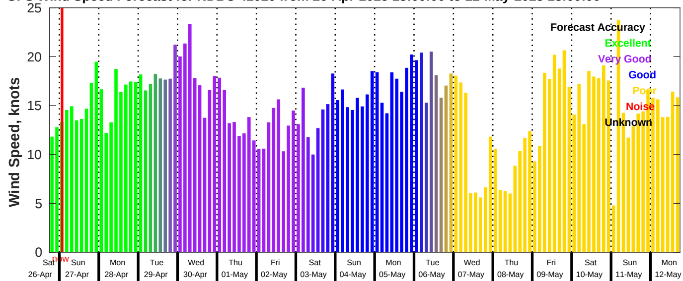
GFS Wind Speed Forecast for NDBC 42020 from 26-Apr-2025 18:00:00 to 12-May-2025 18:00:00
