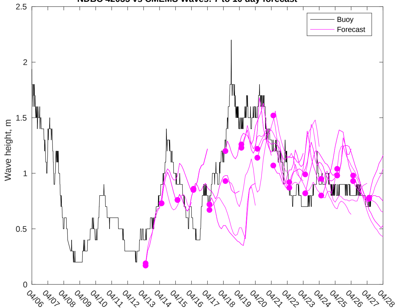
NDBC 42035 vs CMEMS Waves: 7 to 10 day forecast
