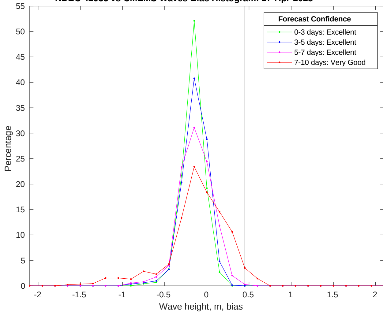
NDBC 42035 vs CMEMS Waves Bias Histogram: 27-Apr-2025
