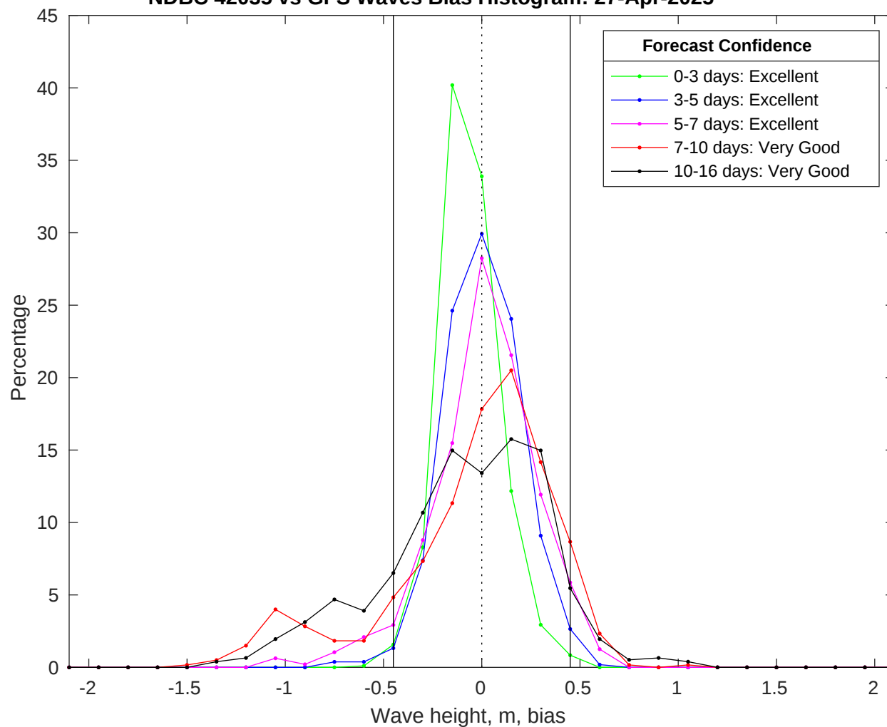
NDBC 42035 vs GFS Waves Bias Histogram: 27-Apr-2025
