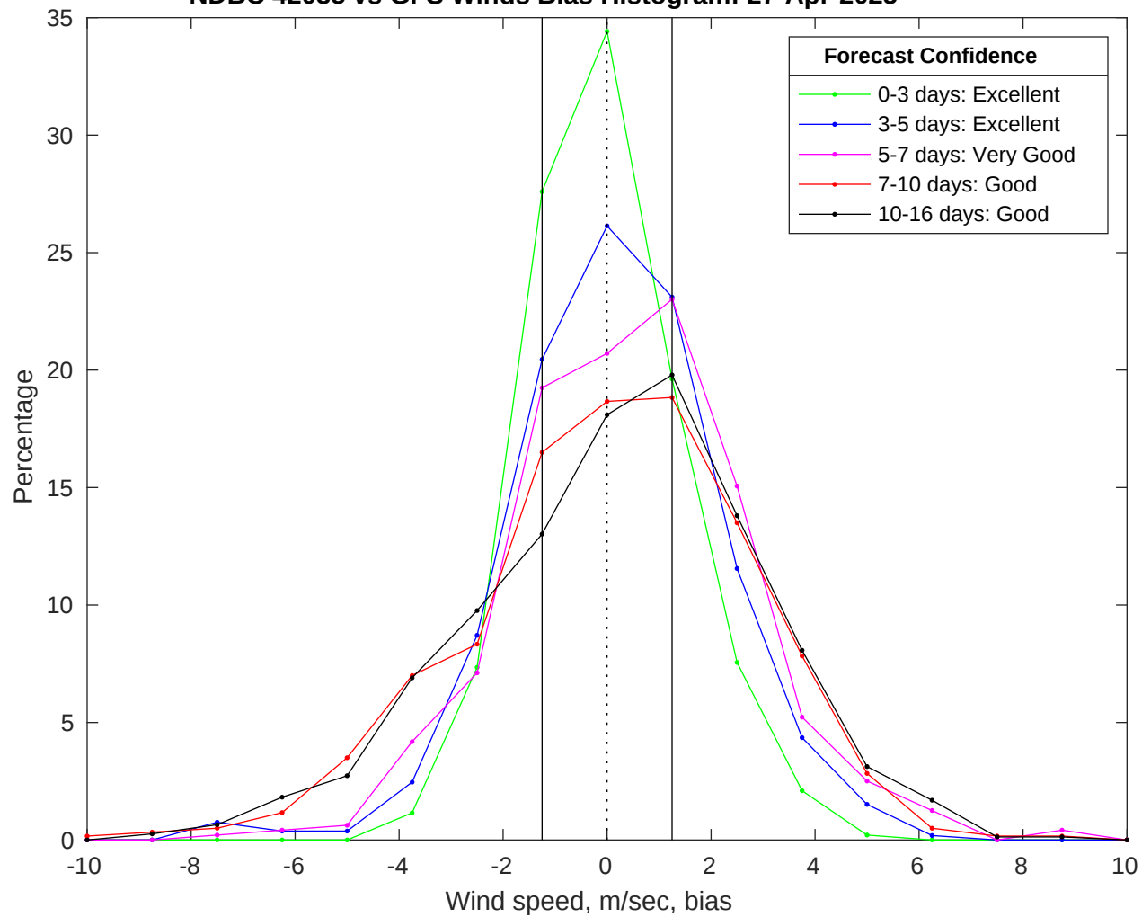
NDBC 42035 vs GFS Winds Bias Histogram: 27-Apr-2025
