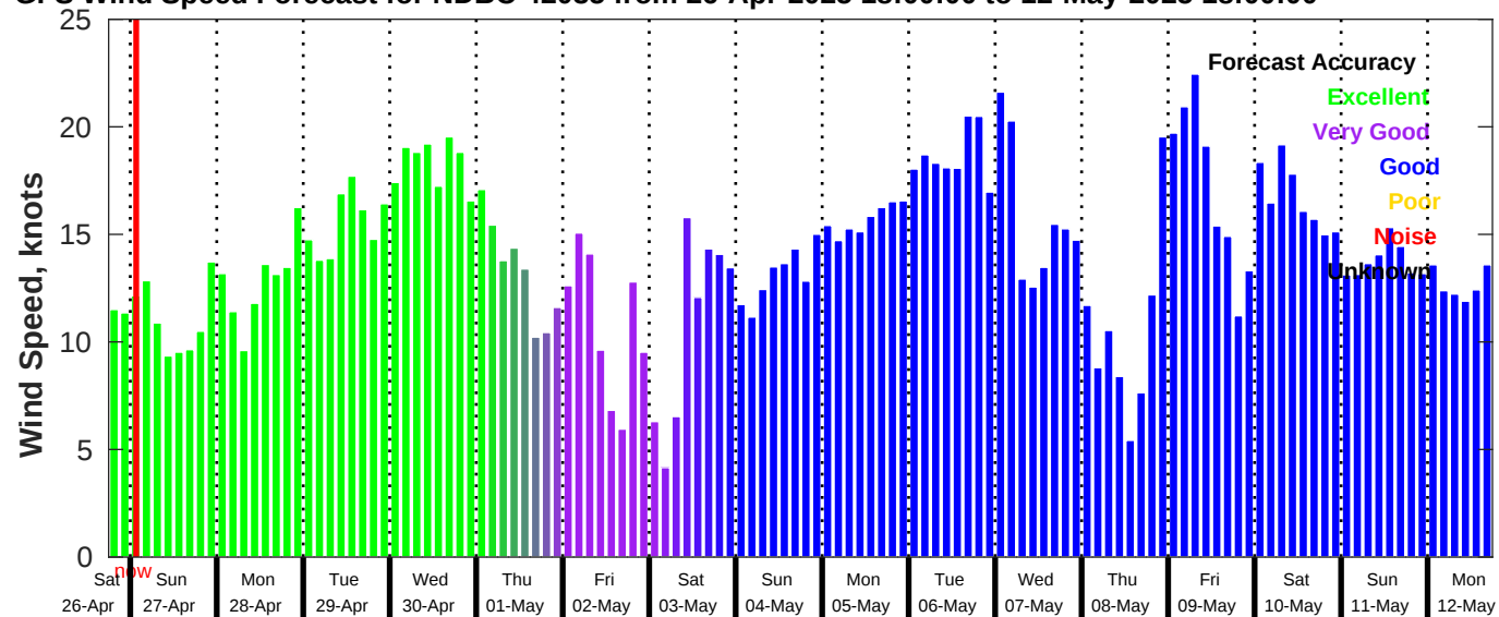
GFS Wind Speed Forecast for NDBC 42035 from 26-Apr-2025 18:00:00 to 12-May-2025 18:00:00
