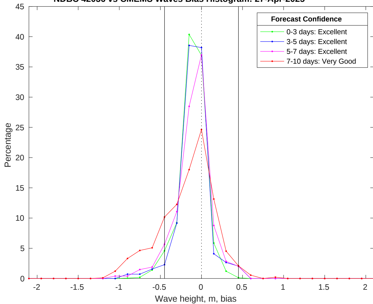
NDBC 42036 vs CMEMS Waves Bias Histogram: 27-Apr-2025
