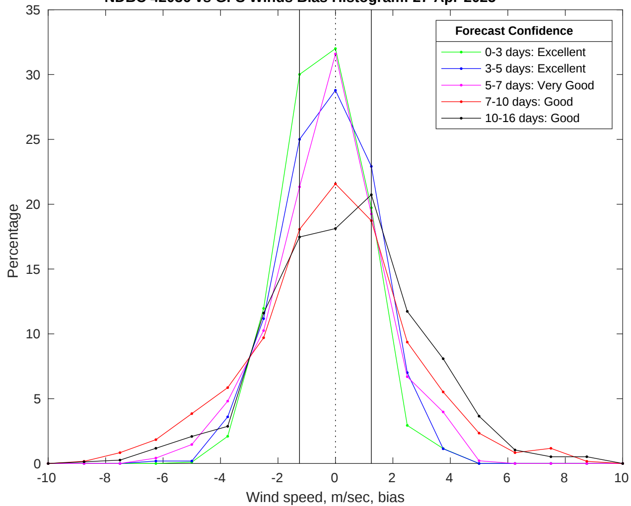
NDBC 42036 vs GFS Winds Bias Histogram: 27-Apr-2025
