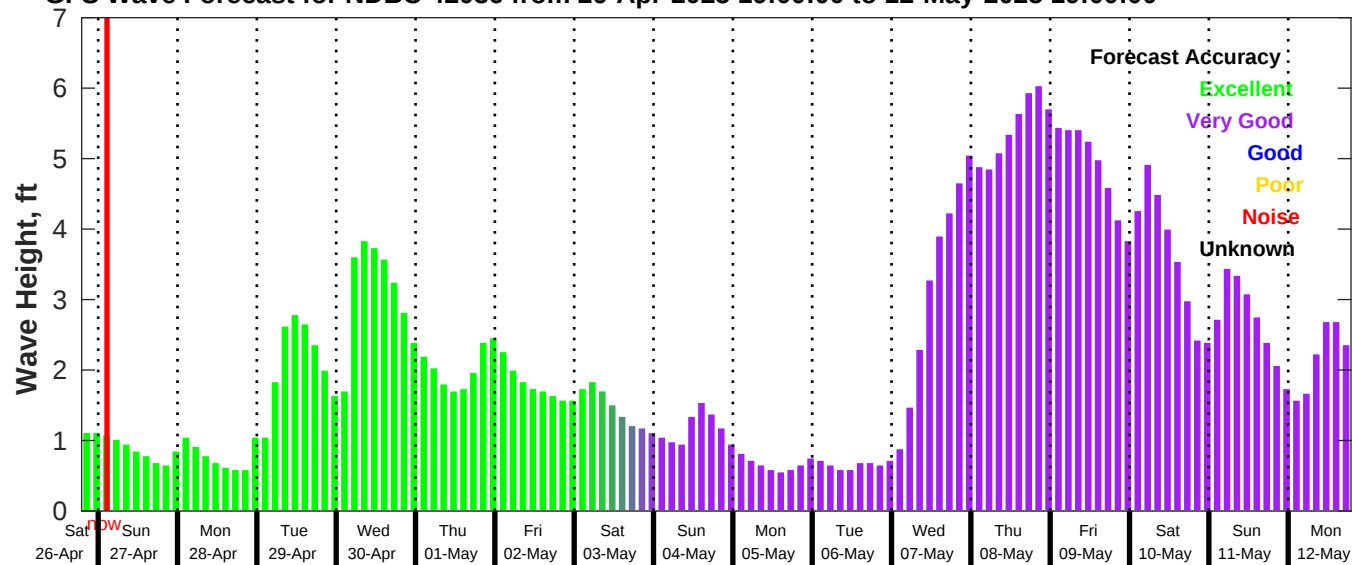
GFS Wave Forecast for NDBC 42036 from 26-Apr-2025 19:00:00 to 12-May-2025 19:00:00
