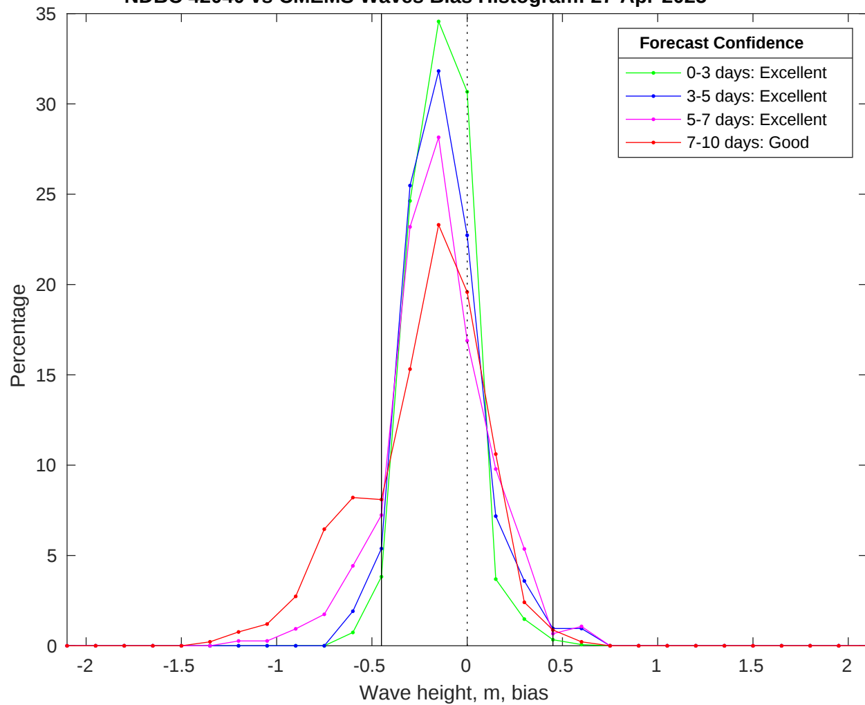
NDBC 42040 vs CMEMS Waves Bias Histogram: 27-Apr-2025
