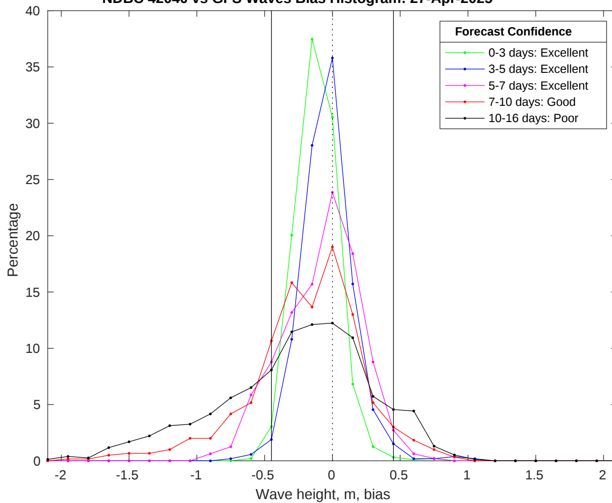
NDBC 42040 vs GFS Waves Bias Histogram: 27-Apr-2025
