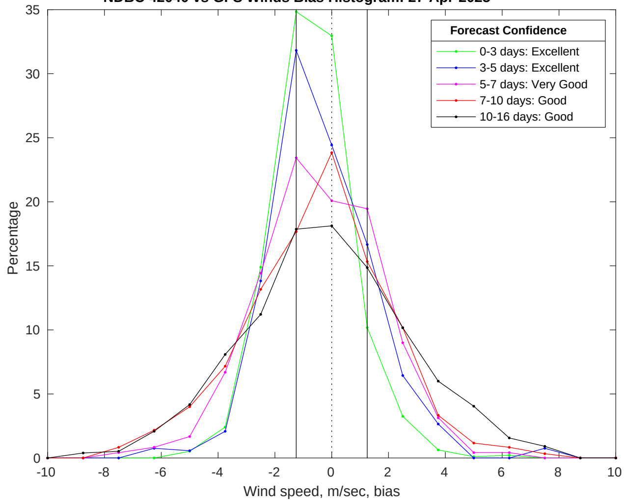
NDBC 42040 vs GFS Winds Bias Histogram: 27-Apr-2025
