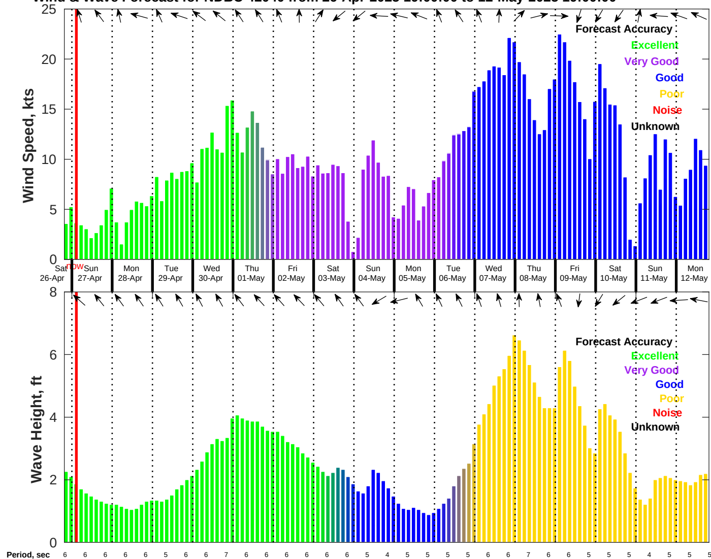
Wind & Wave Forecast for NDBC 42040 from 26-Apr-2025 19:00:00 to 12-May-2025 19:00:00
