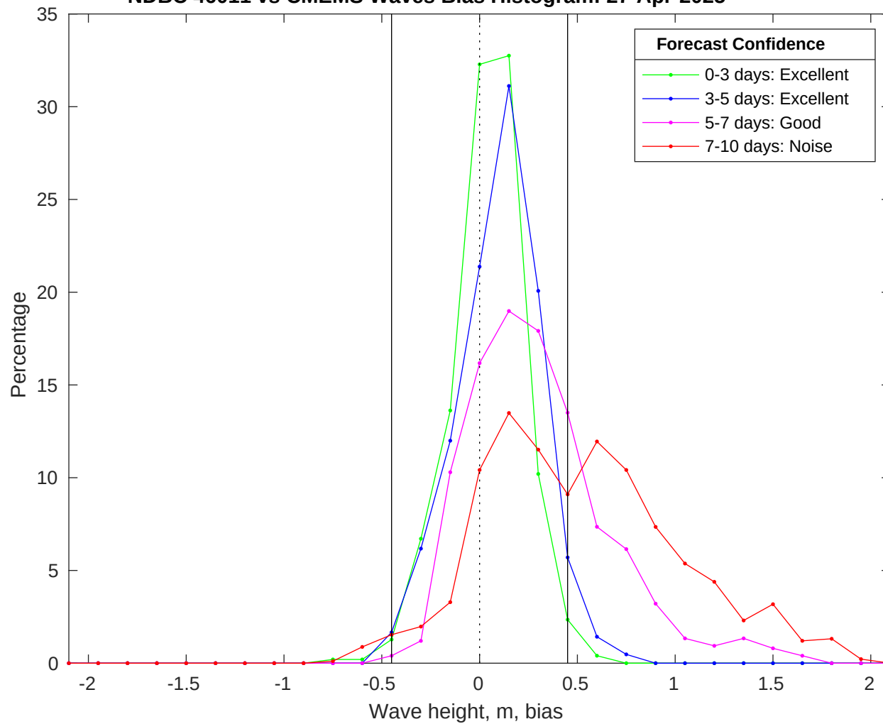
NDBC 46011 vs CMEMS Waves Bias Histogram: 27-Apr-2025
