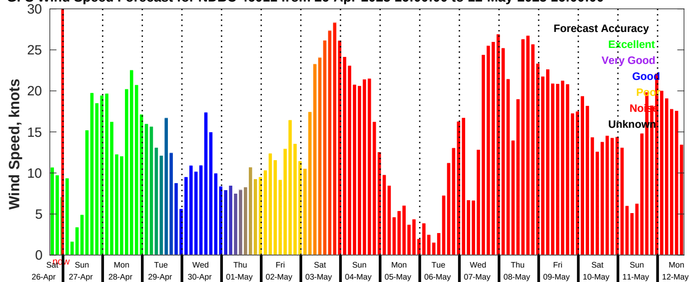
GFS Wind Speed Forecast for NDBC 46011 from 26-Apr-2025 16:00:00 to 12-May-2025 16:00:00
