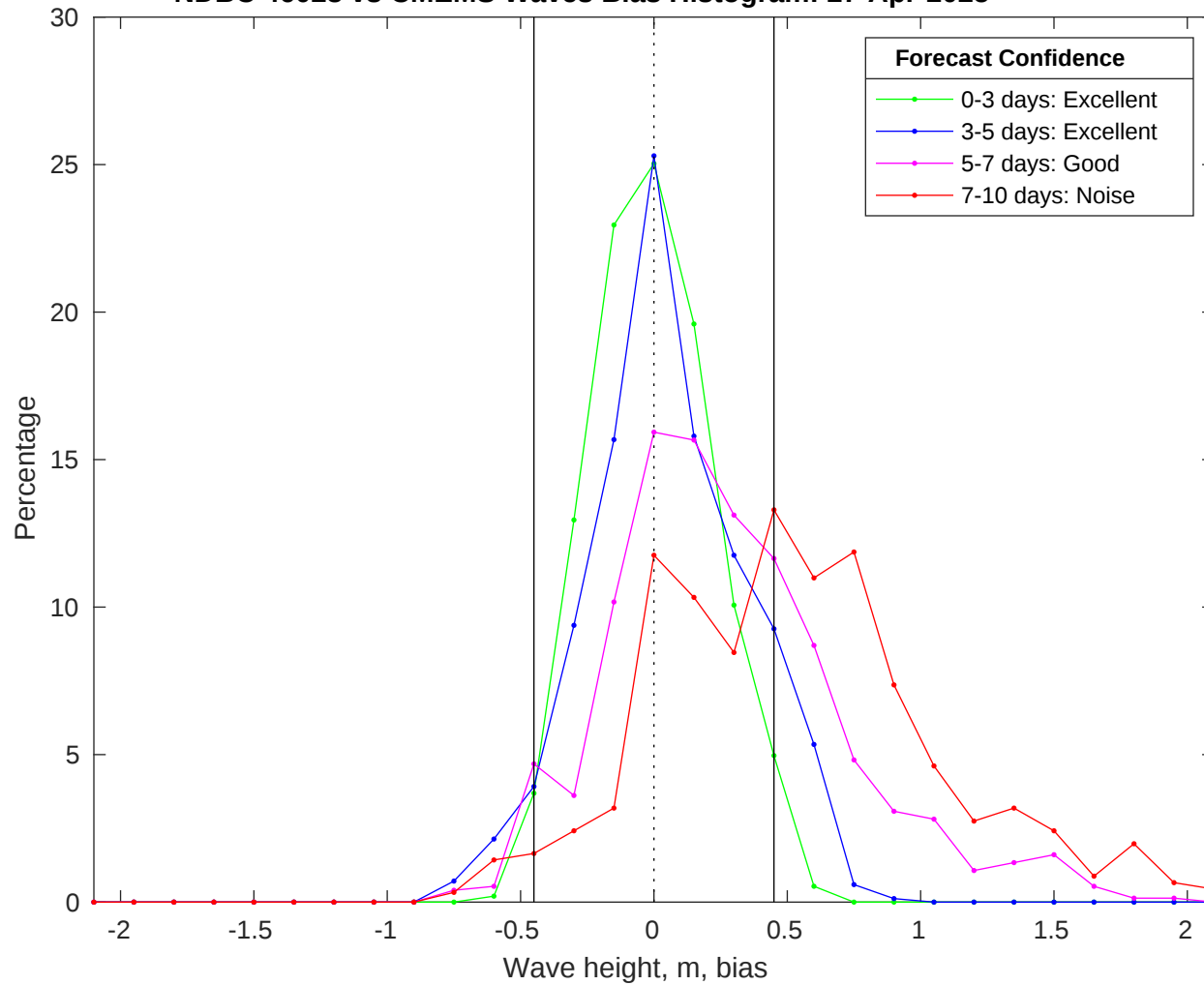
NDBC 46028 vs CMEMS Waves Bias Histogram: 27-Apr-2025
