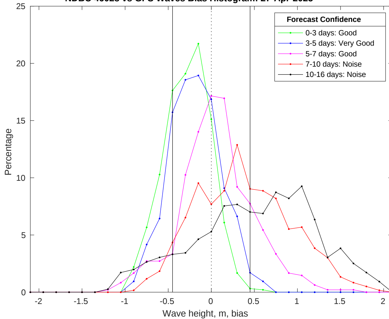
NDBC 46028 vs GFS Waves Bias Histogram: 27-Apr-2025
