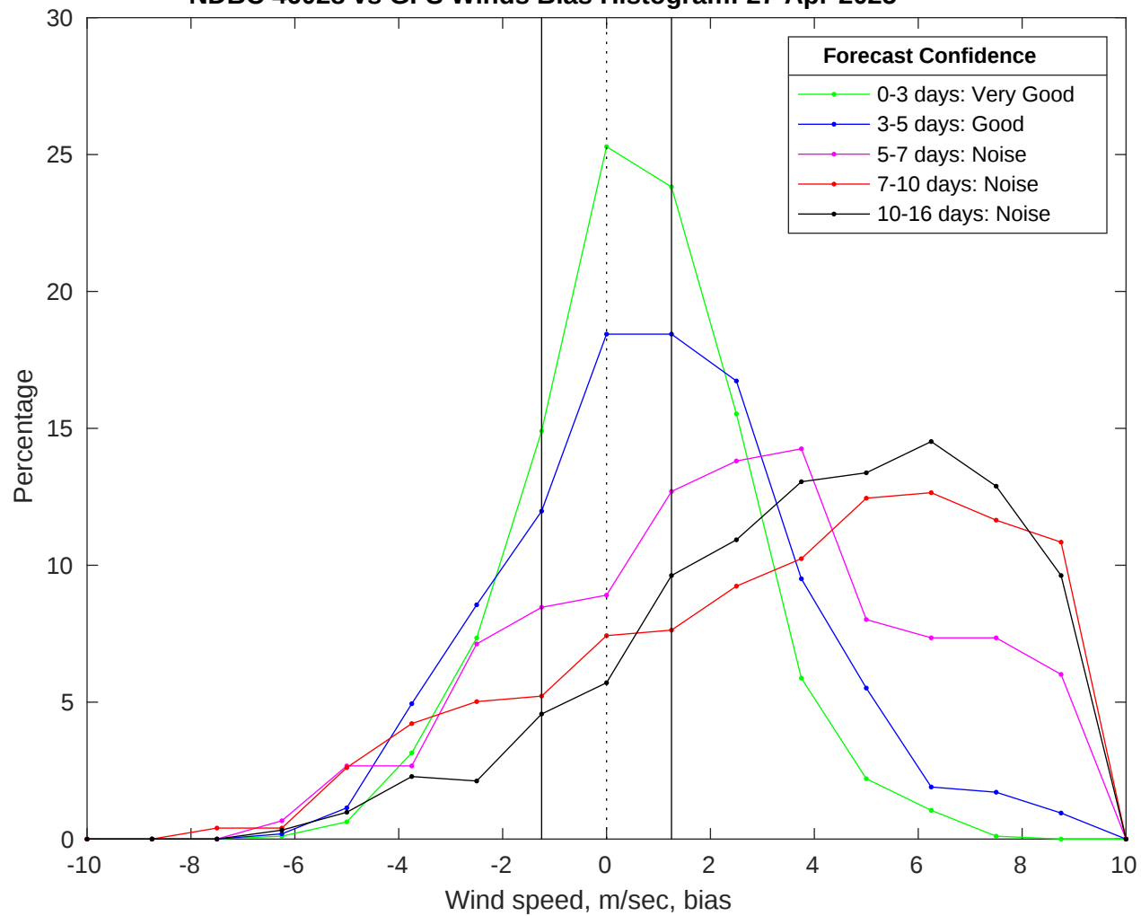
NDBC 46028 vs GFS Winds Bias Histogram: 27-Apr-2025
