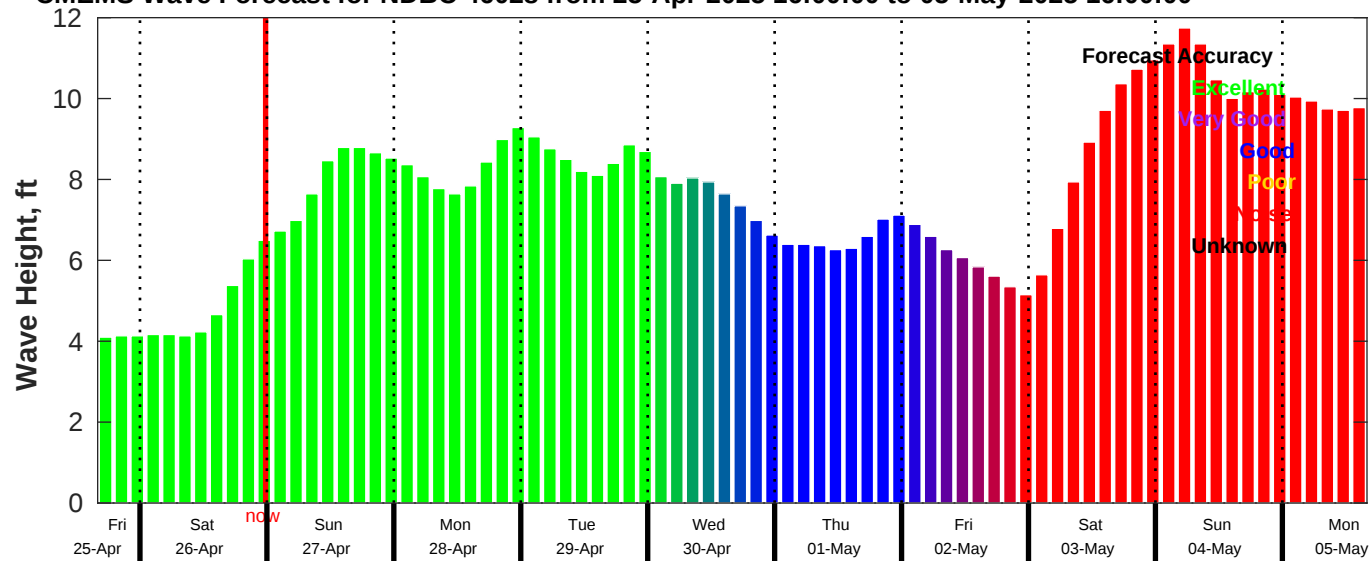
CMEMS Wave Forecast for NDBC 46028 from 25-Apr-2025 16:00:00 to 05-May-2025 16:00:00
