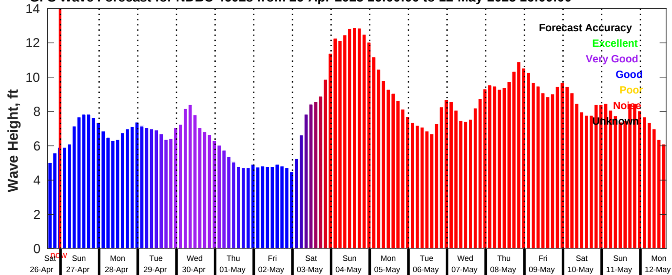
GFS Wave Forecast for NDBC 46028 from 26-Apr-2025 16:00:00 to 12-May-2025 16:00:00
