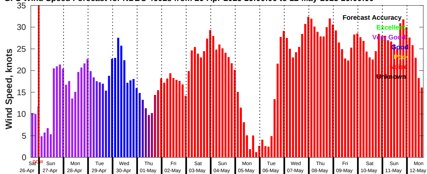
GFS Wind Speed Forecast for NDBC 46028 from 26-Apr-2025 16:00:00 to 12-May-2025 16:00:00
