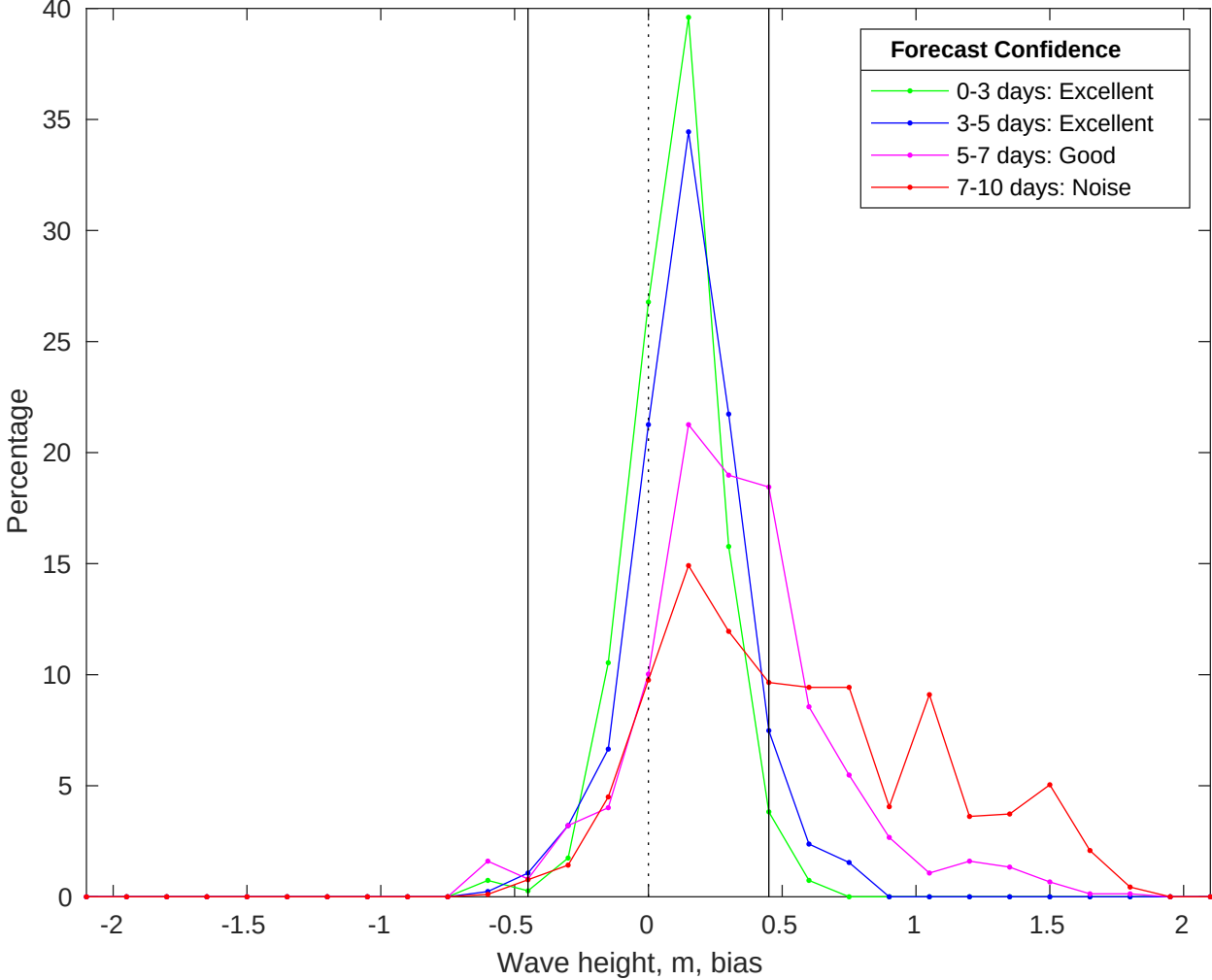
NDBC 46054 vs CMEMS Waves Bias Histogram: 27-Apr-2025
