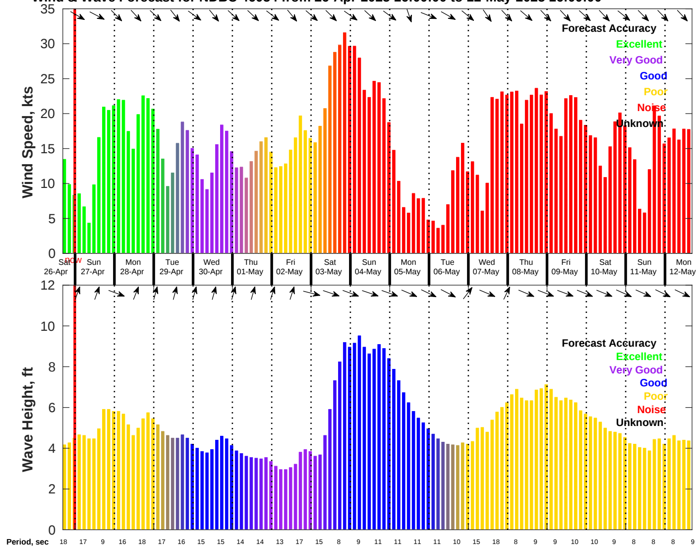
Wind & Wave Forecast for NDBC 46054 from 26-Apr-2025 16:00:00 to 12-May-2025 16:00:00
