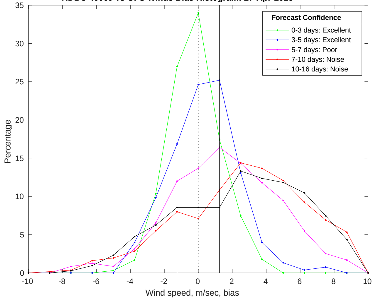
NDBC 46069 vs GFS Winds Bias Histogram: 27-Apr-2025
