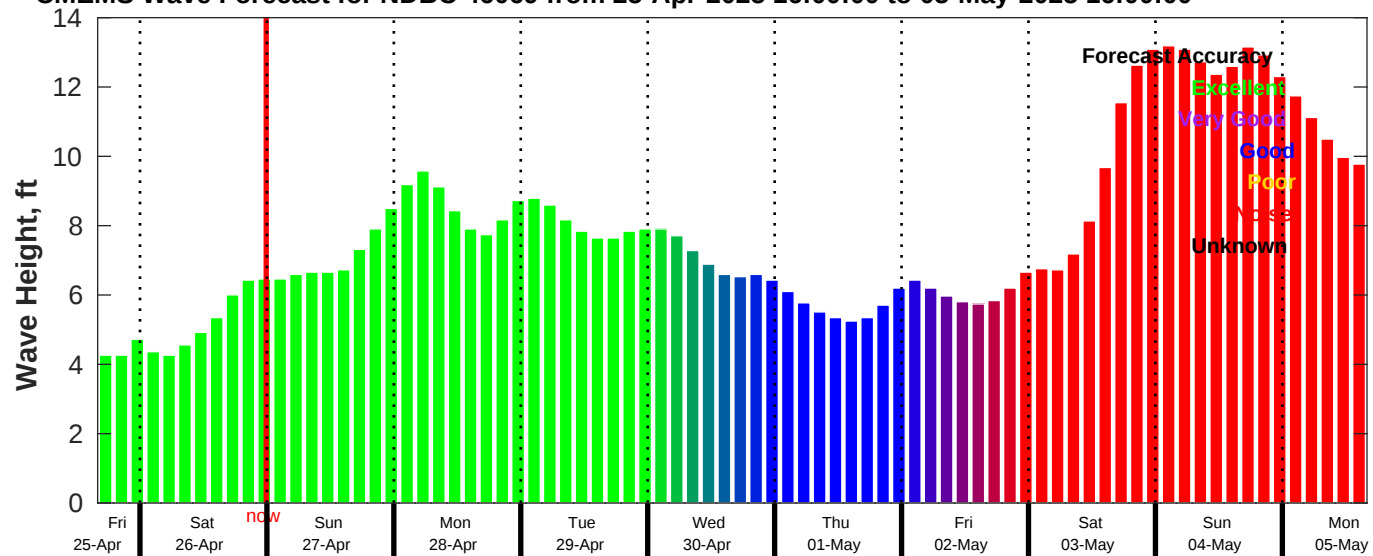
CMEMS Wave Forecast for NDBC 46069 from 25-Apr-2025 16:00:00 to 05-May-2025 16:00:00
