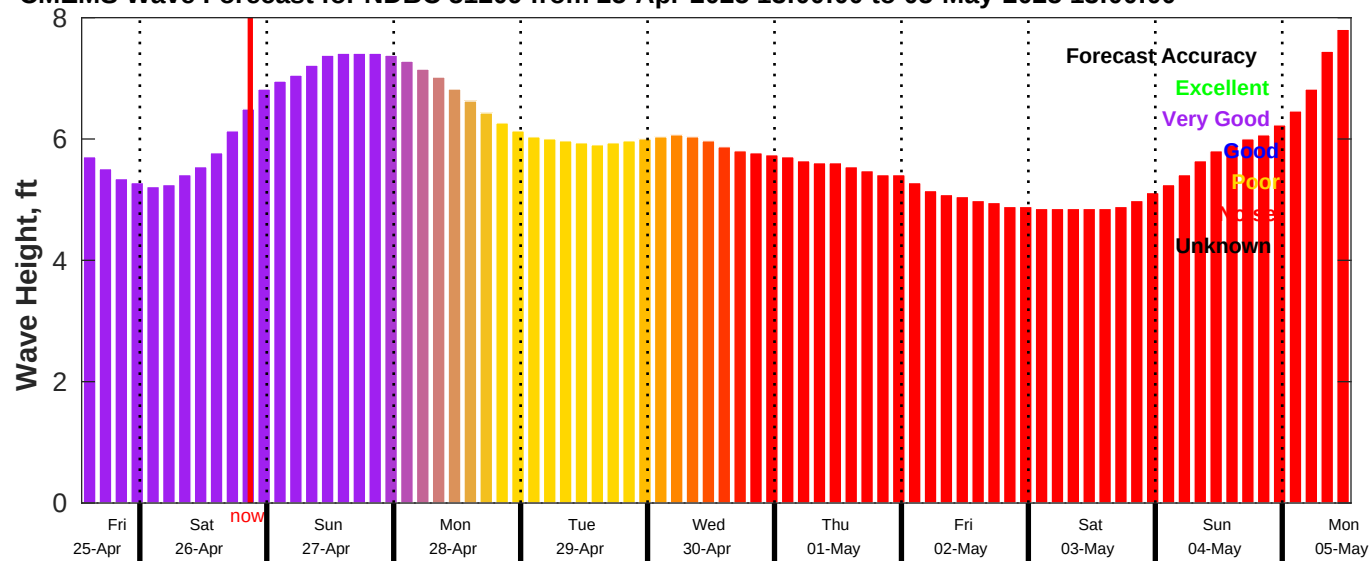
CMEMS Wave Forecast for NDBC 51209 from 25-Apr-2025 13:00:00 to 05-May-2025 13:00:00
