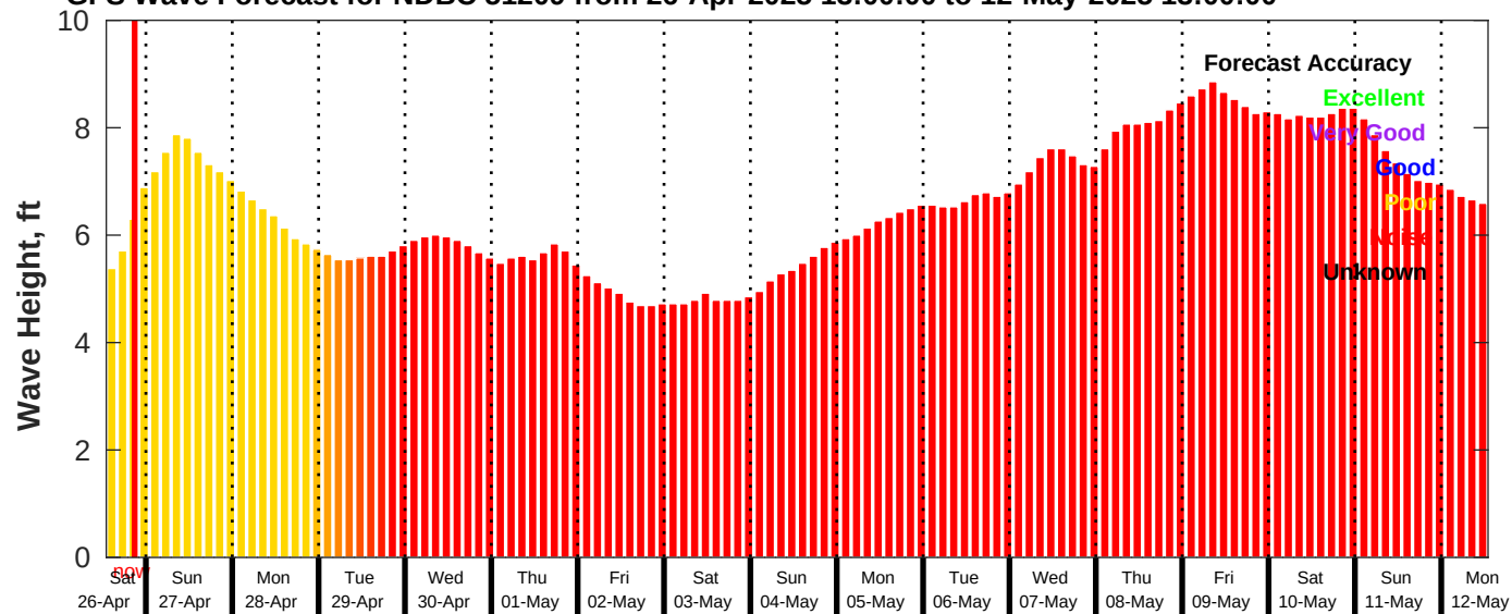
GFS Wave Forecast for NDBC 51209 from 26-Apr-2025 13:00:00 to 12-May-2025 13:00:00
