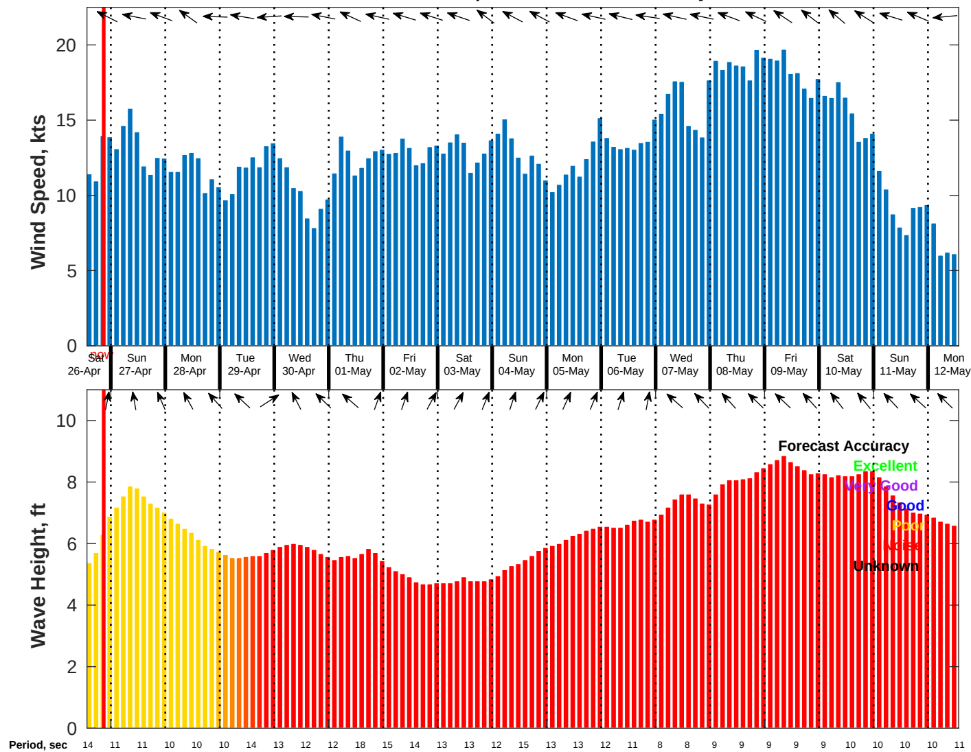
Wind & Wave Forecast for NDBC 51209 from 26-Apr-2025 13:00:00 to 12-May-2025 13:00:00
