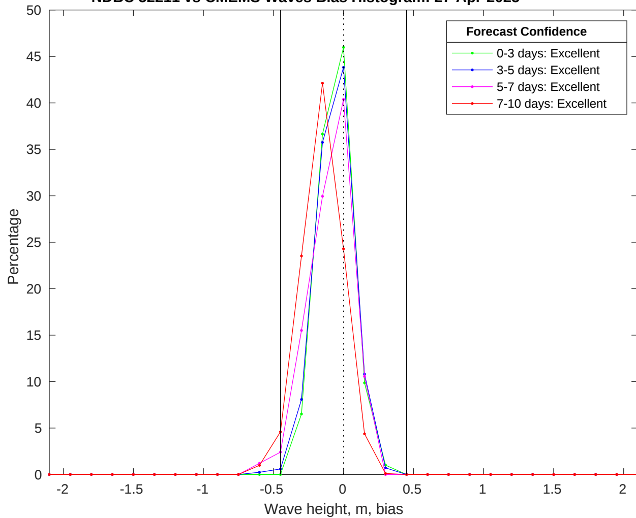
NDBC 52211 vs CMEMS Waves Bias Histogram: 27-Apr-2025
