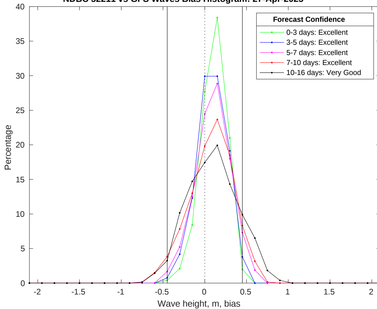
NDBC 52211 vs GFS Waves Bias Histogram: 27-Apr-2025
