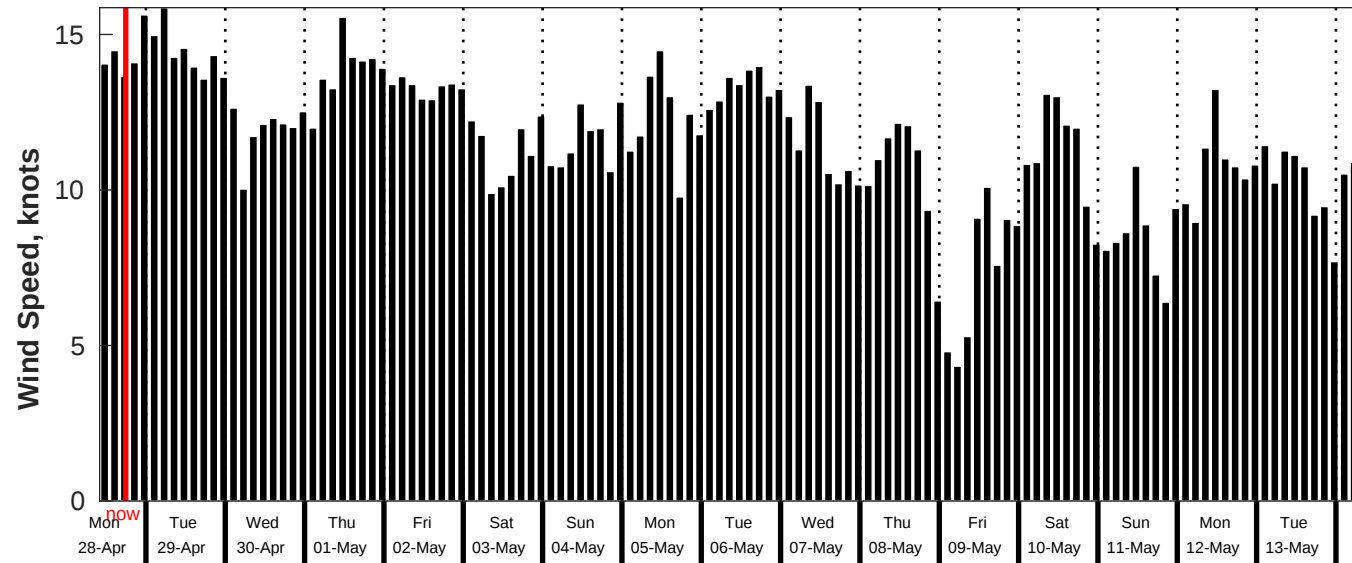
GFS Wind Speed Forecast for NDBC 52211 from 27-Apr-2025 10:00:00 to 13-May-2025 10:00:00
