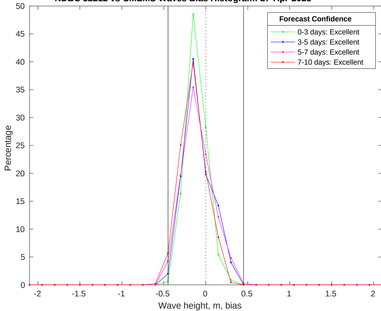
NDBC 52212 vs CMEMS Waves Bias Histogram: 27-Apr-2025
