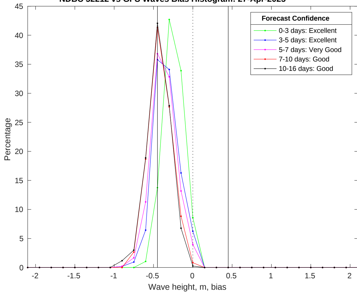
NDBC 52212 vs GFS Waves Bias Histogram: 27-Apr-2025
