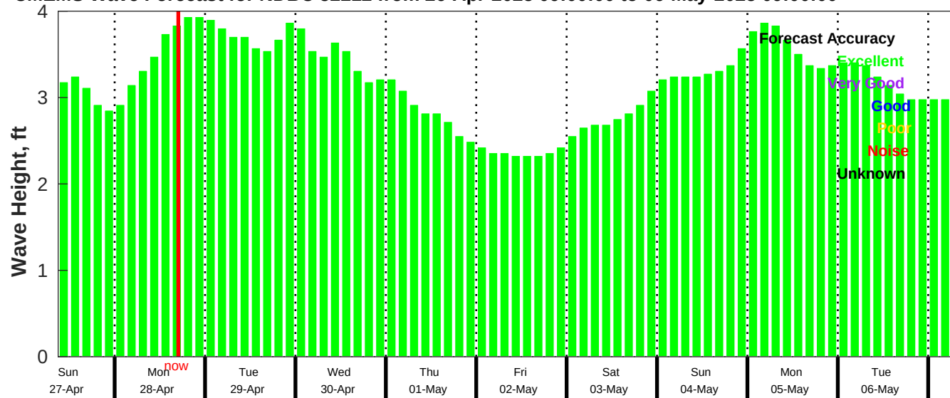
CMEMS Wave Forecast for NDBC 52212 from 26-Apr-2025 09:00:00 to 06-May-2025 09:00:00
