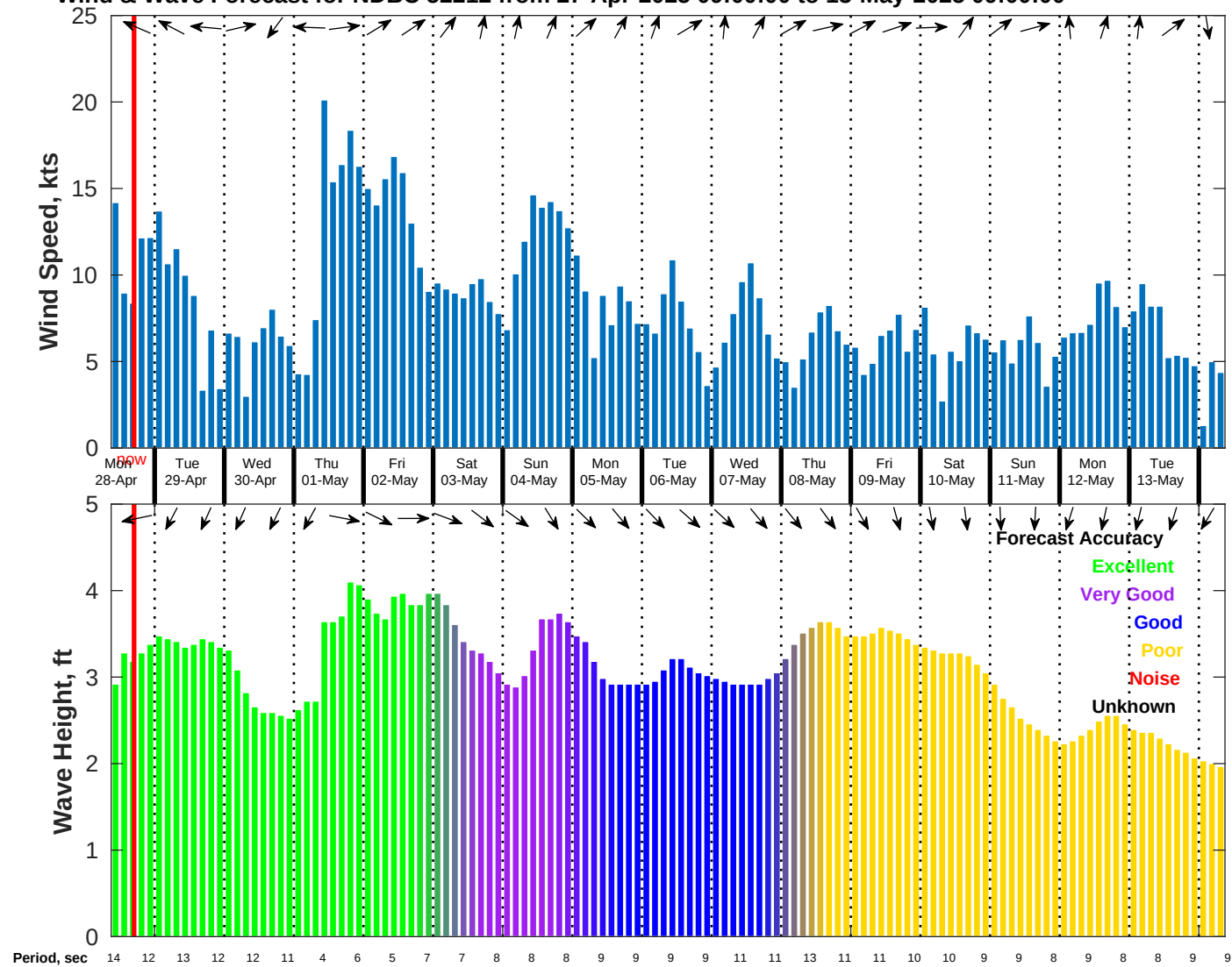
Wind & Wave Forecast for NDBC 52212 from 27-Apr-2025 09:00:00 to 13-May-2025 09:00:00
