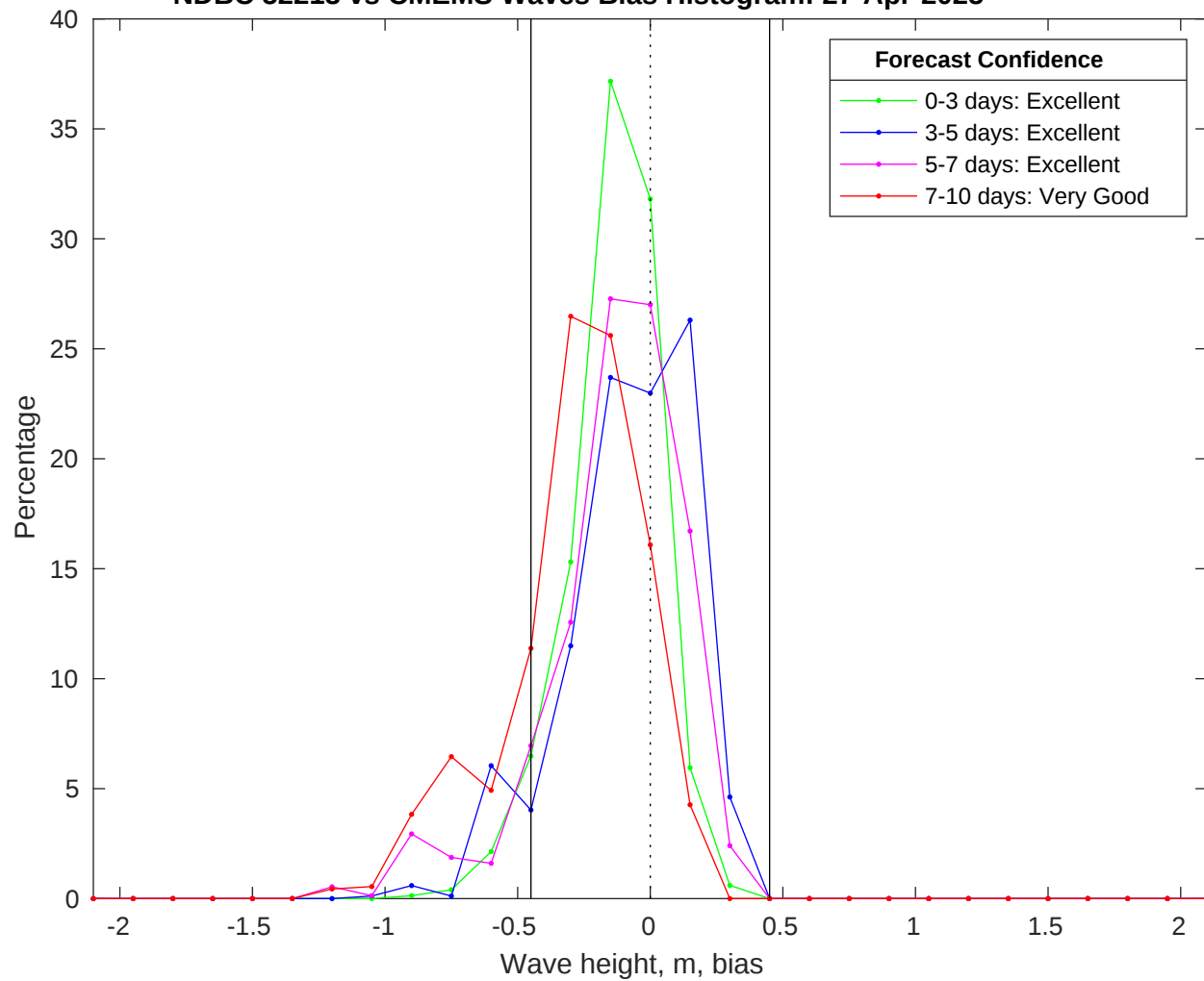
NDBC 52213 vs CMEMS Waves Bias Histogram: 27-Apr-2025
