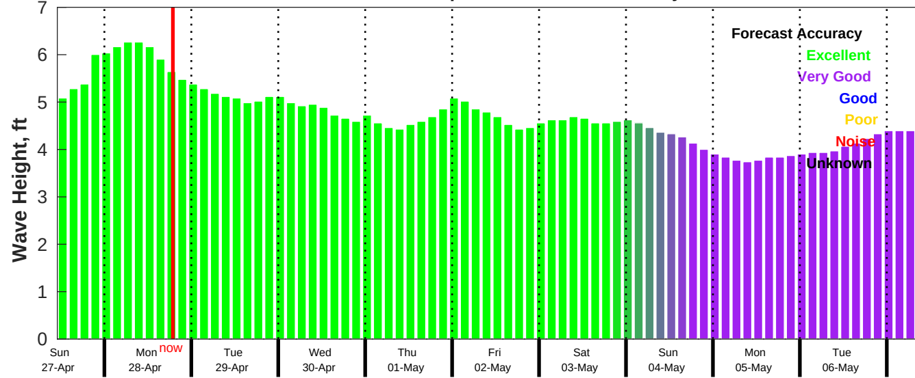
CMEMS Wave Forecast for NDBC 52213 from 26-Apr-2025 11:00:00 to 06-May-2025 11:00:00
