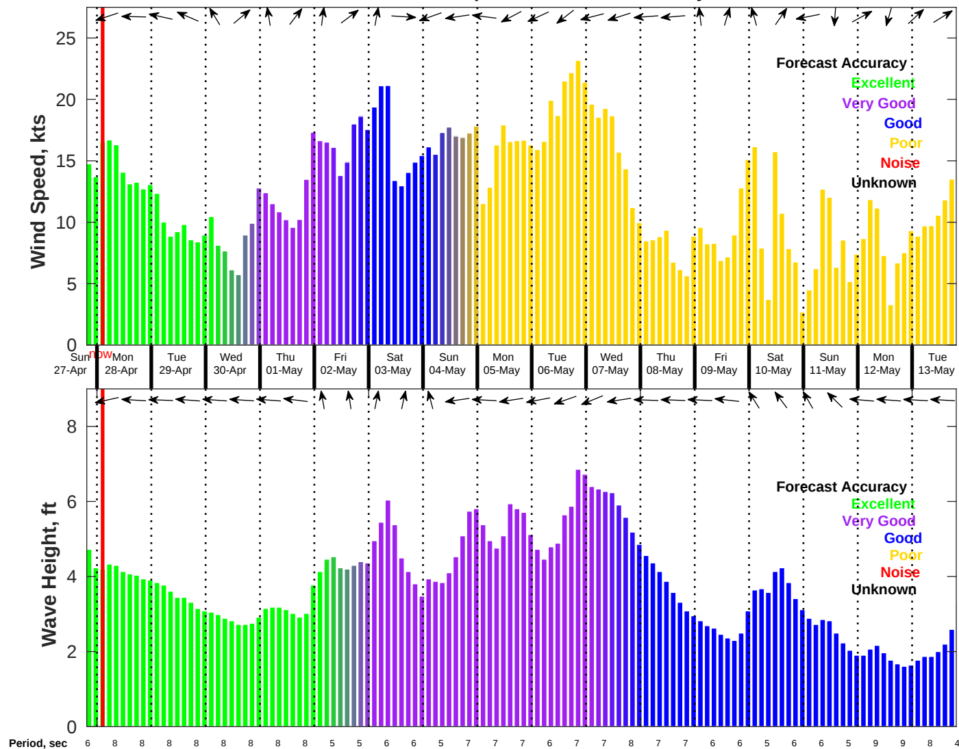
Wind & Wave Forecast for NDBC 41004 from 27-Apr-2025 19:00:00 to 13-May-2025 19:00:00
