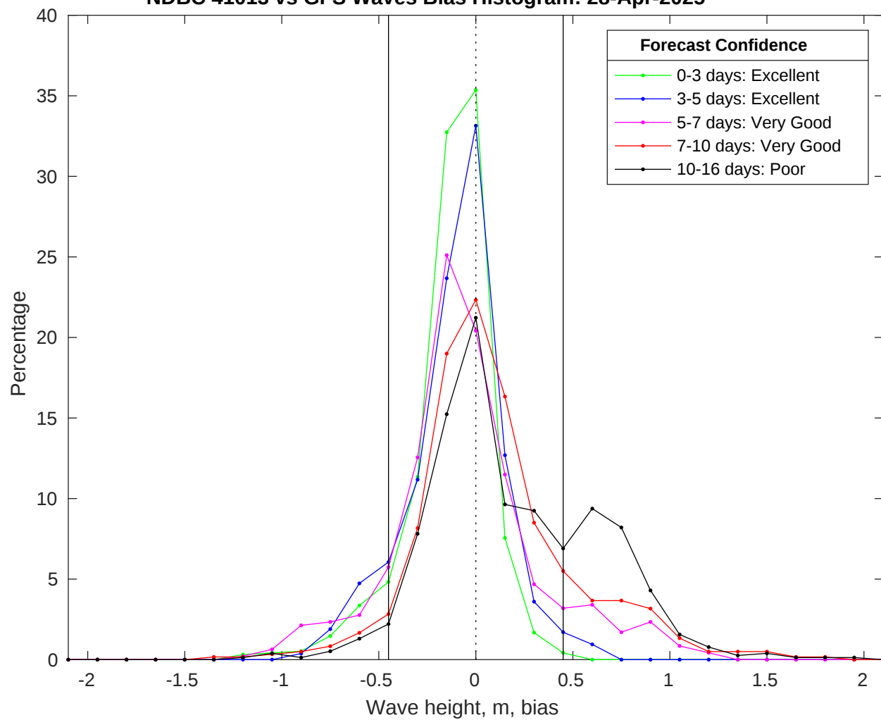
NDBC 41013 vs GFS Waves Bias Histogram: 28-Apr-2025
