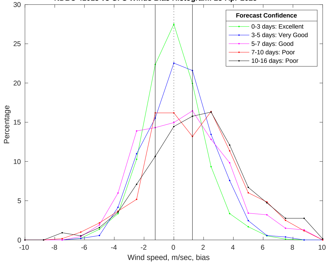
NDBC 41013 vs GFS Winds Bias Histogram: 28-Apr-2025
