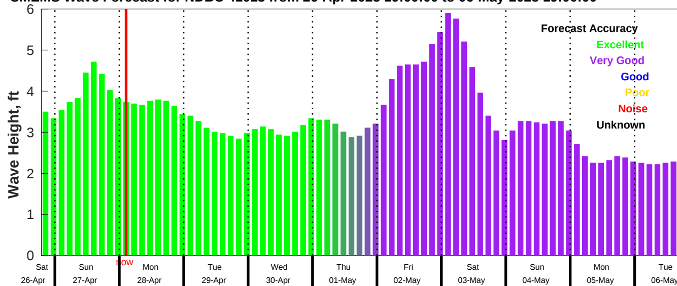
CMEMS Wave Forecast for NDBC 41013 from 26-Apr-2025 19:00:00 to 06-May-2025 19:00:00
