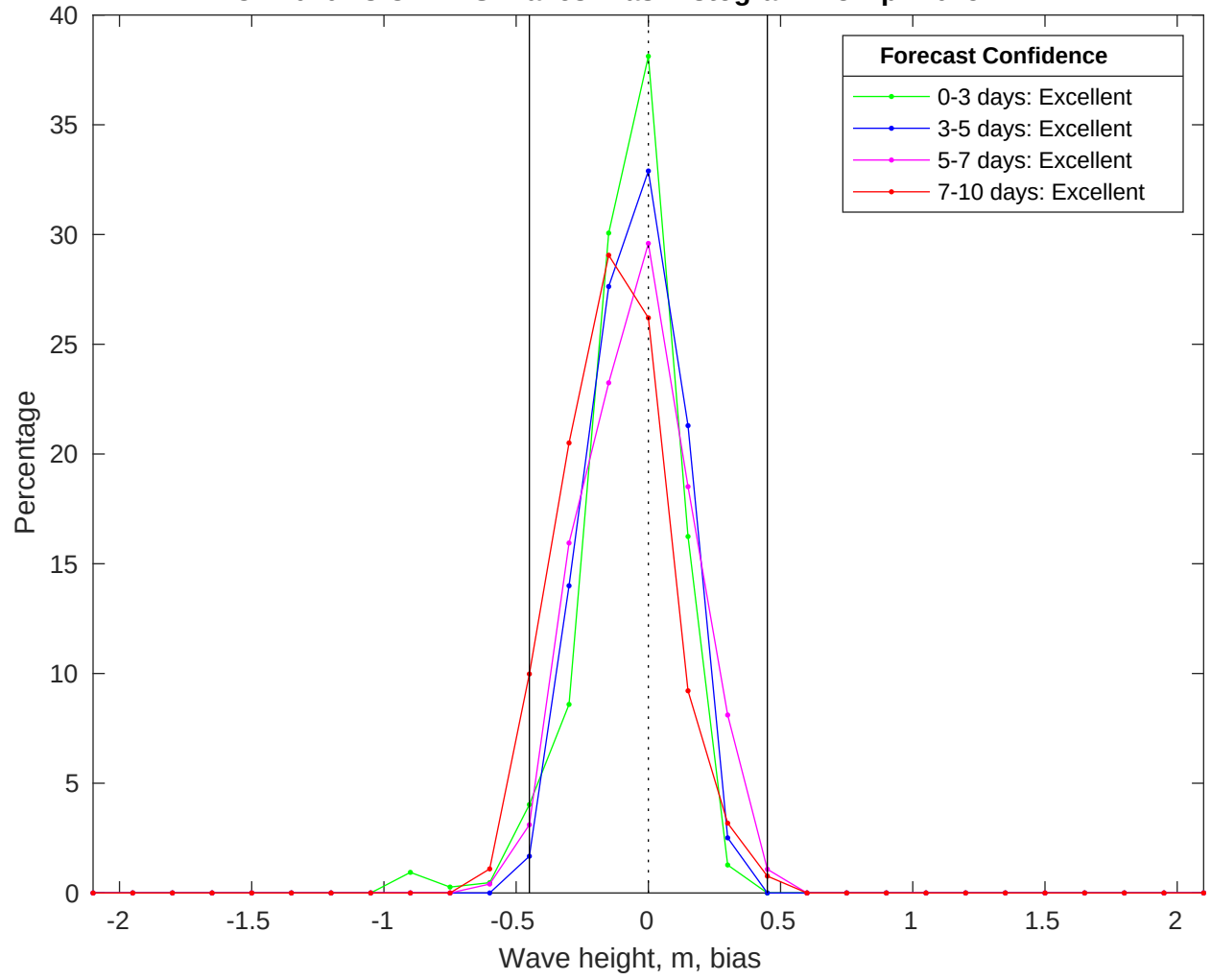
NDBC 41040 vs CMEMS Waves Bias Histogram: 28-Apr-2025
