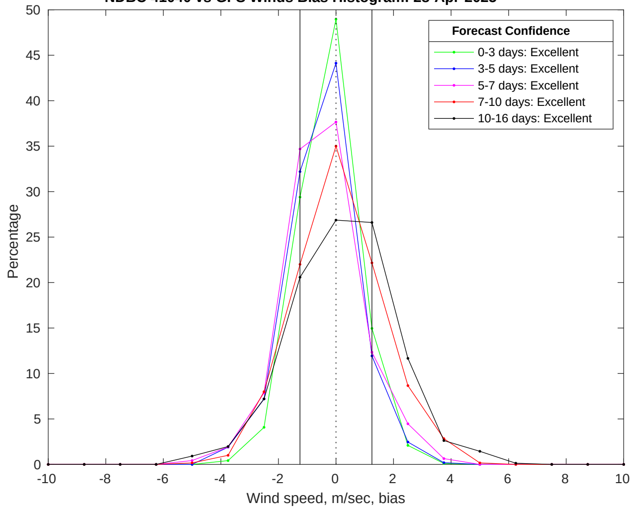
NDBC 41040 vs GFS Winds Bias Histogram: 28-Apr-2025
