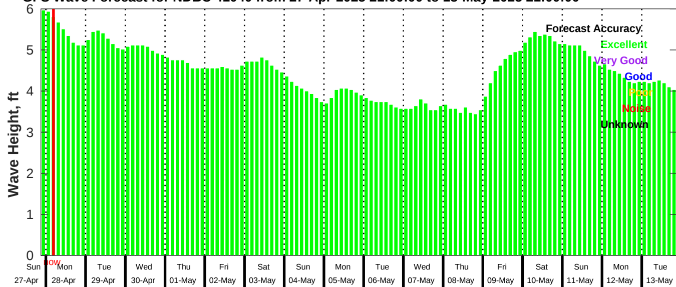
GFS Wave Forecast for NDBC 41040 from 27-Apr-2025 21:00:00 to 13-May-2025 21:00:00
