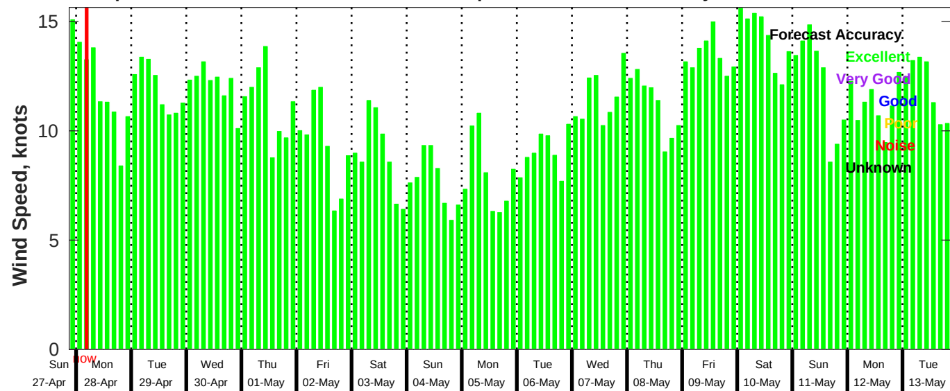
GFS Wind Speed Forecast for NDBC 41040 from 27-Apr-2025 21:00:00 to 13-May-2025 21:00:00
