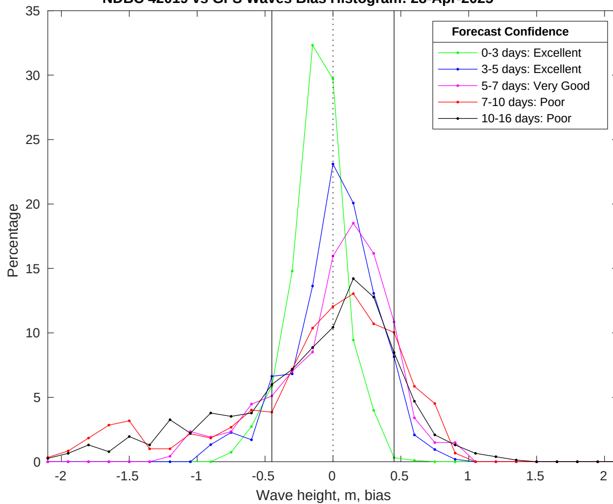
NDBC 42019 vs GFS Waves Bias Histogram: 28-Apr-2025
